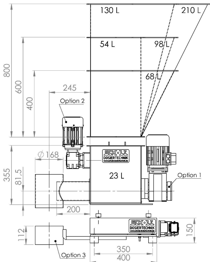
Differential-Dosierwaage RATIO Loss-in-Weight-Feeder RATIO
